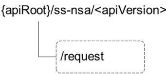
Figure 7.7.1.3.1-1: Custom operation URI structure of the SS_NetworkSliceAdaptation API
