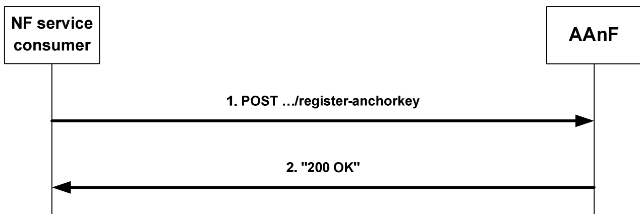
Figure 4.2.2.2.2-1: Registration of AKMA related key material
