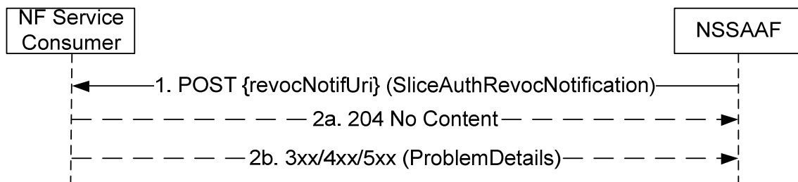
Figure 5.2.2.4.1-1: Revocation Notification
