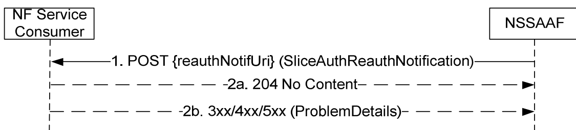
Figure 5.2.2.3.1-1: Re-authentication Notification
