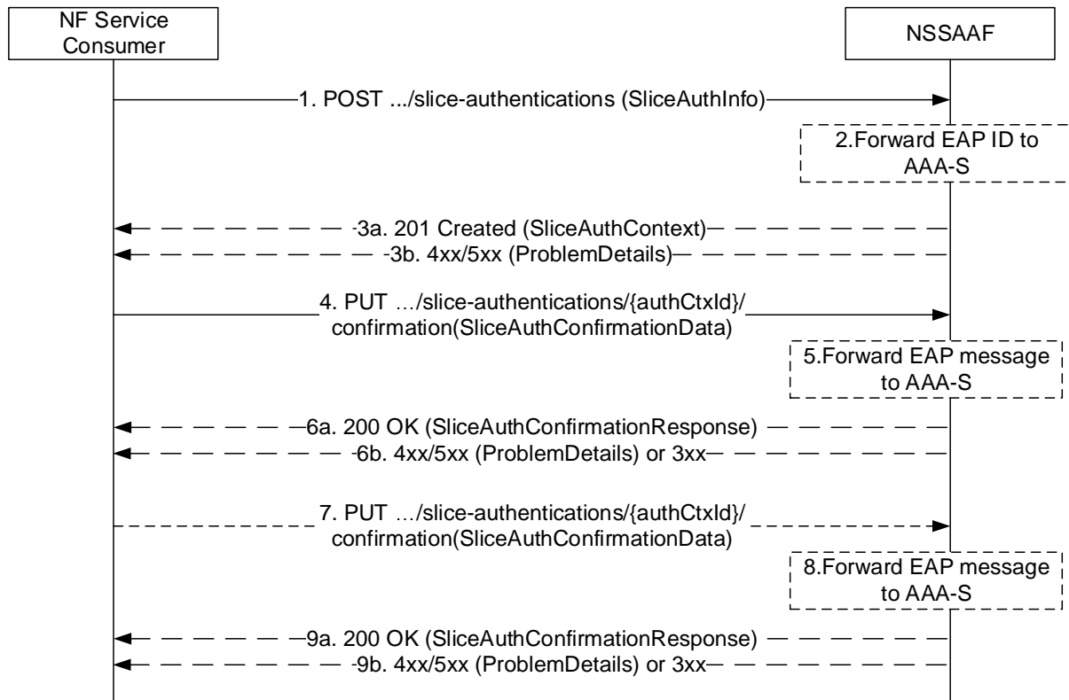
Figure 5.2.2.1-1: Slice-Specific Authentication and Authorization
