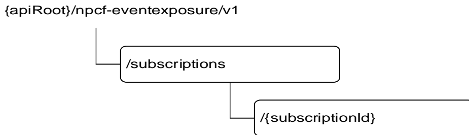
Figure 5.3.1-1: Resource URI structure of the Npcf_EventExposure API
