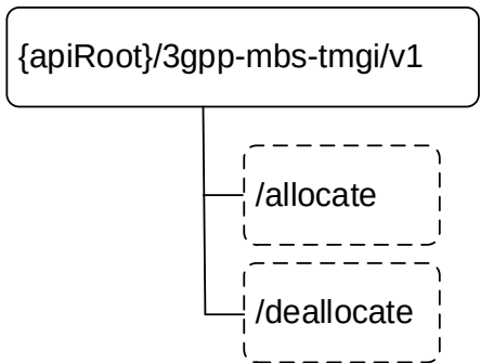
Figure 5.19.3.1-1: Custom operation URI structure of the MBSTMGI API
