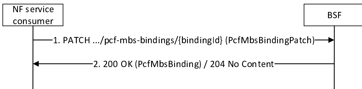
Figure 4.2.5.4-1: NF service consumer update an existing PCF for an MBS Session binding information
