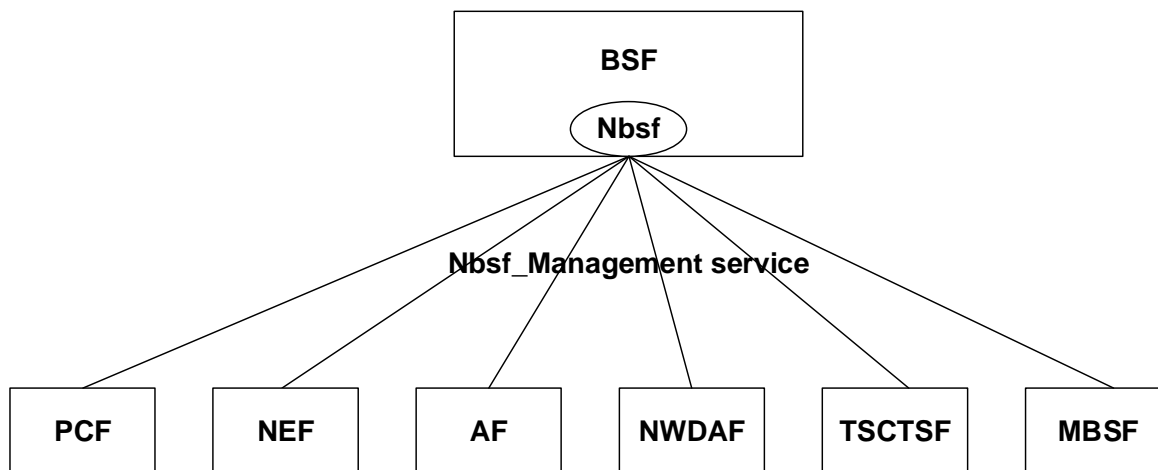
Figure 4.1.2-1: Reference Architecture for the Nbsf_Management service; SBI representation
