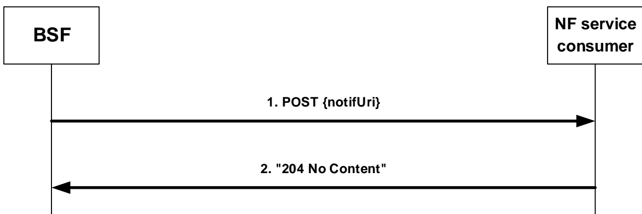
Figure 4.2.8.2-1: Notification about subscribed events
