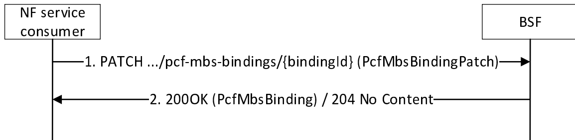
Figure 4.2.5.4-1: NF service consumer update an existing PCF for a UE binding information
