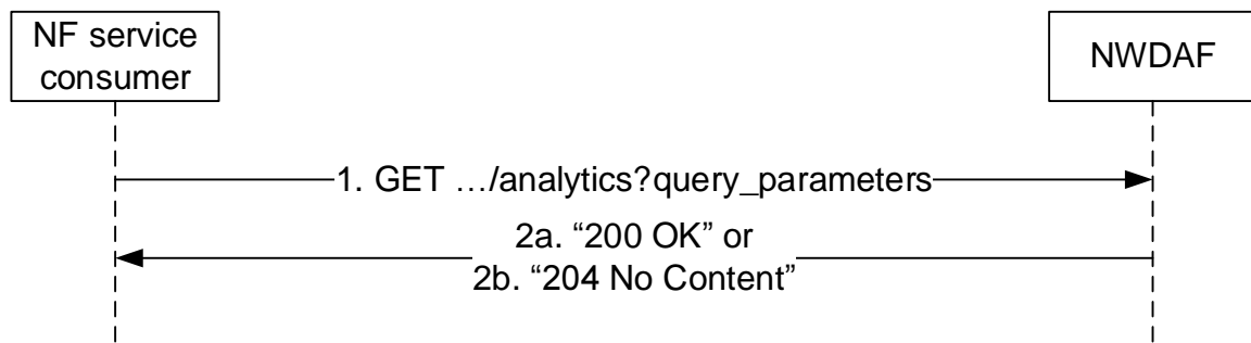
Figure 4.3.2.2-1: Requesting a NWDaf Analytics information
