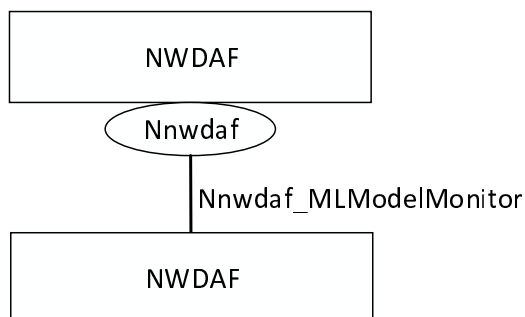
Figure 4.7.1.2-1: Reference Architecture for the Nnwdafl_MLModelMonitor Service; SBI representation
