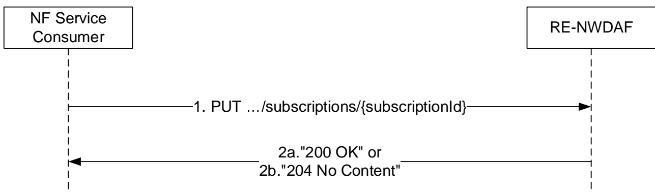
Figure 4.8.2.2.3-1: NF service consumer updates subscription to notifications
