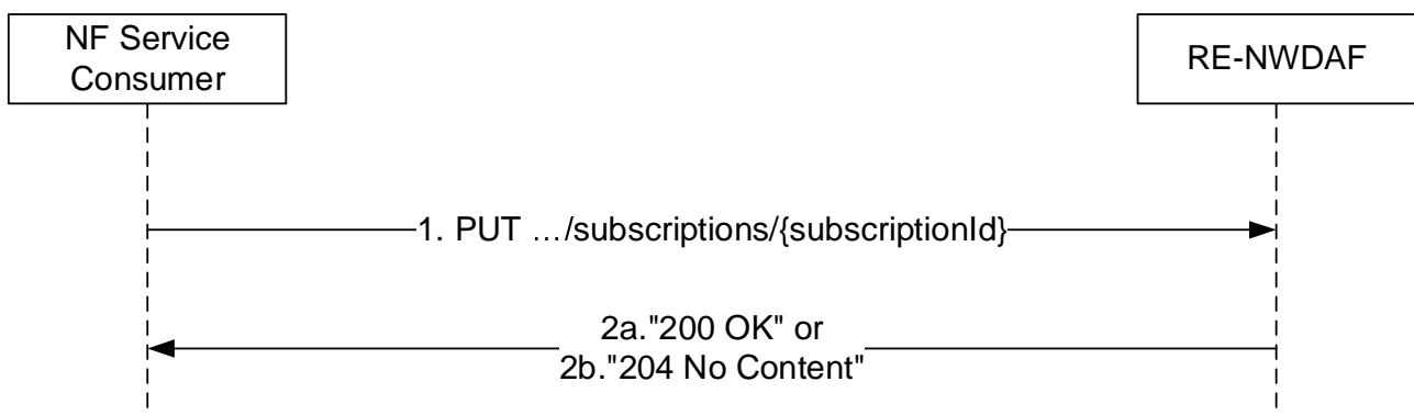
Figure 4.9.2.2.3-1: NF service consumer updates subscription to notifications
