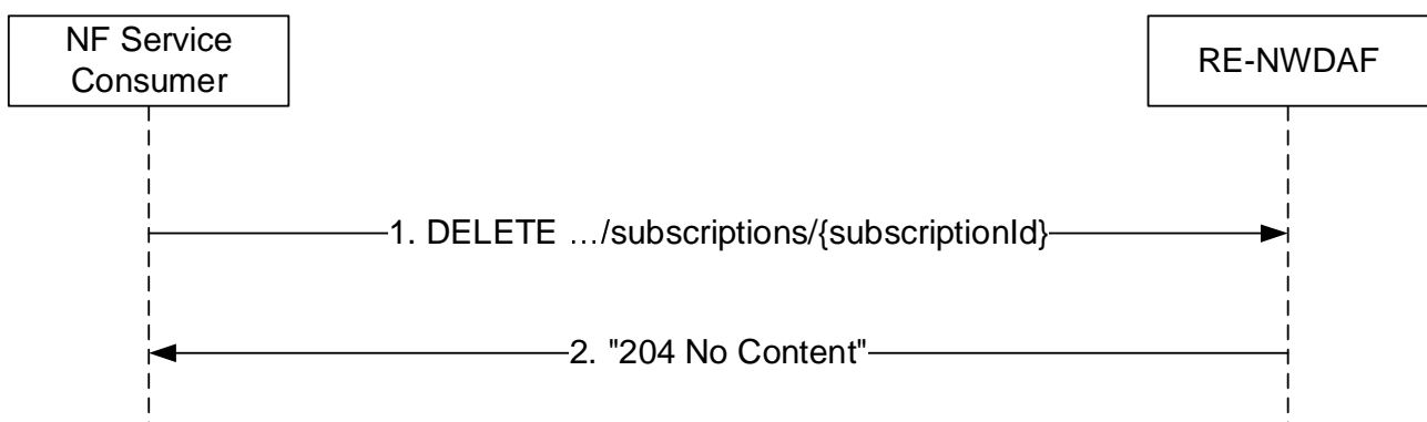
Figure 4.9.2.3.2-1: NF service consumer unsubscribes from notifications
