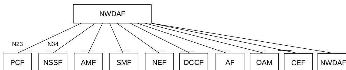
Figure 4.2.1.2-2: Reference Architecture for the Nnwdaf_EventsSubscription Service: reference point representation
