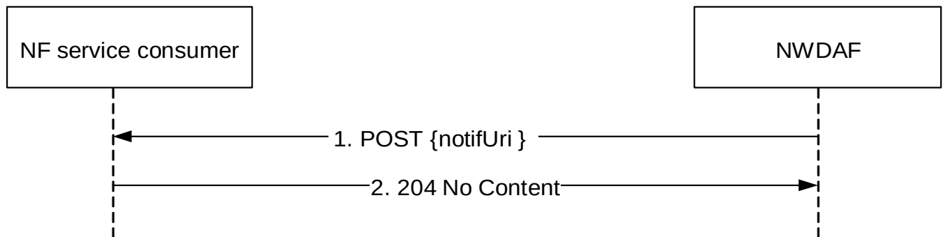
Figure 4.5.2.4.2-1: NWDAF notifies the subscribed event
