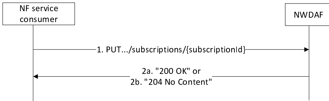
Figure 4.4.2.2.3-1: NF service consumer updates subscription to data notifications
