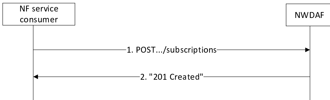
Figure 4.4.2.2.2-1: NF service consumer subscribes to data notifications
