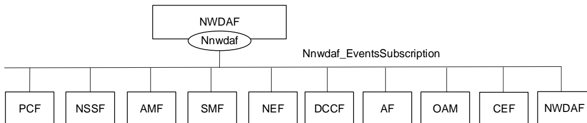
Figure 4.2.1.2-1: Reference Architecture for the Nnwdaq_EventsSubscription Service; SBI representation
