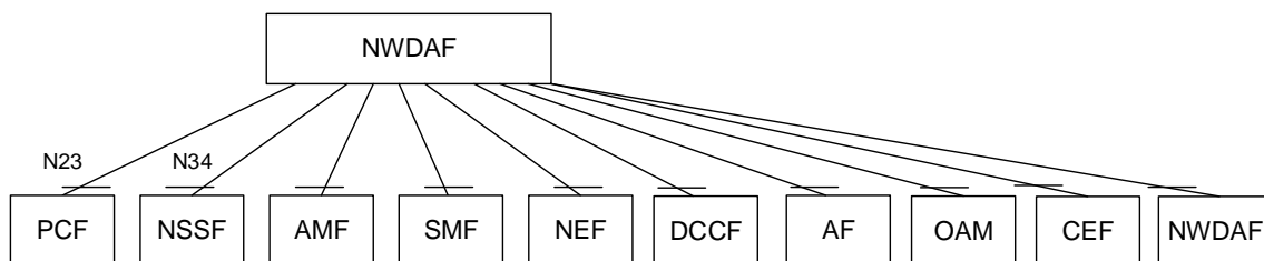
Figure 4.2.1.2-2: Reference Architecture for the Nnwdaq_EventsSubscription Service: reference point representation
