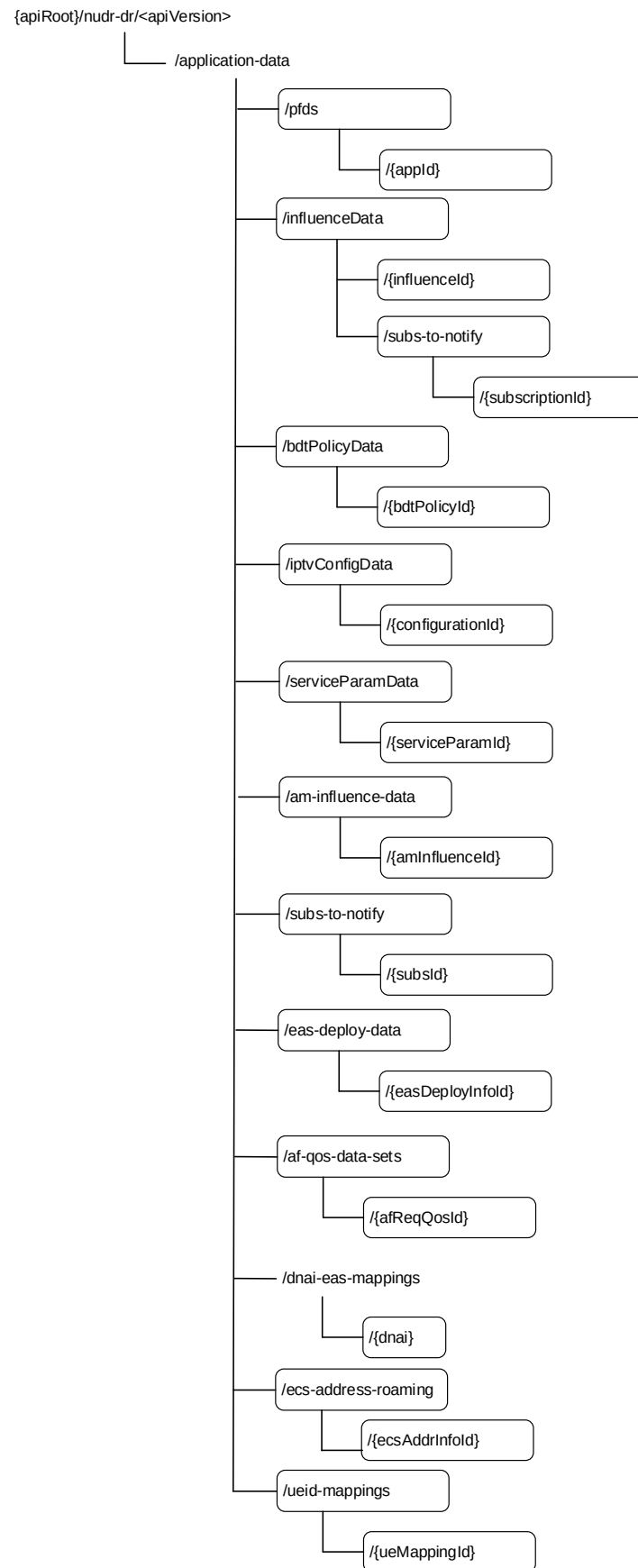
Figure 6.2.2-1: Resource URI structure of the Nudr_DataRepository API for application data
