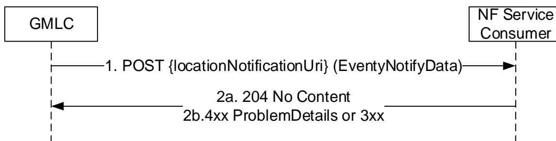
Figure 5.2.2.5.3-1: EventNotify Notification for the UEs in a target group
