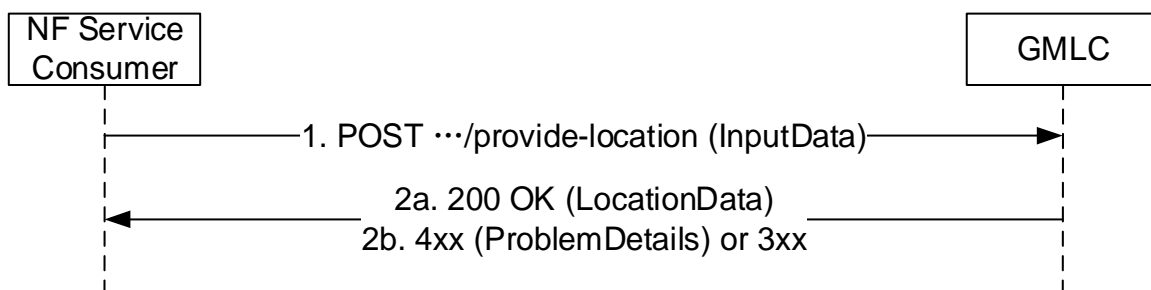
Figure 5.2.2.2.3-1: ProvideLocation Request/Response for a target group
