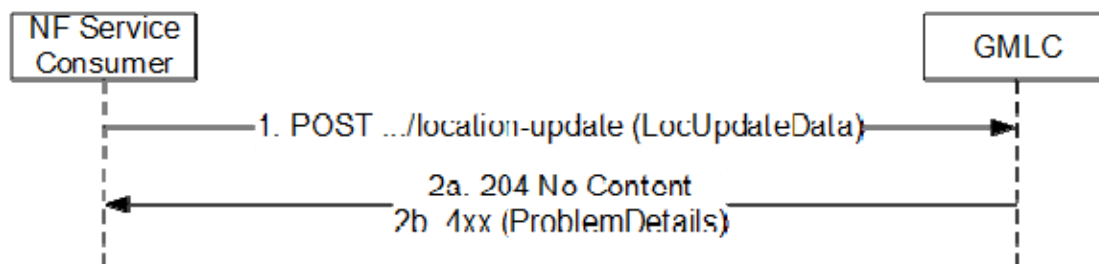
Figure 5.2.2.3.1-1: LocationUpdate Request/Response
