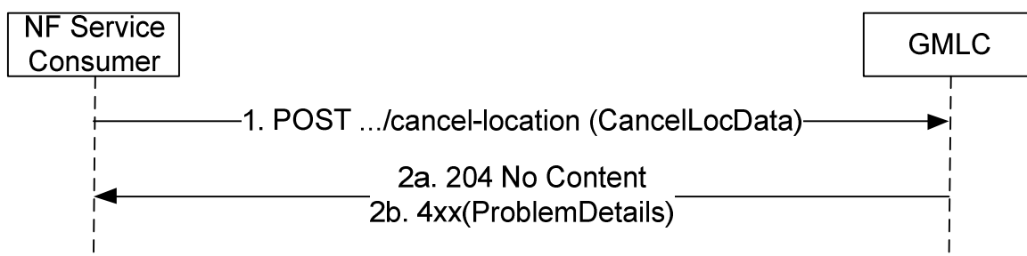
Figure 5.2.2.4.1-1: CancelLocation Request/Response
