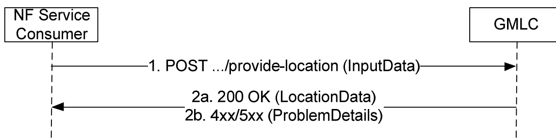
Figure 5.2.2.2.1-1: ProvideLocation Request/Response
