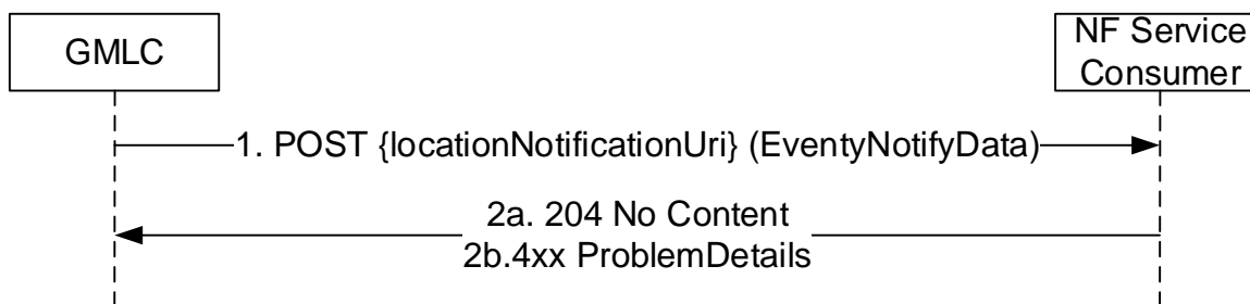
Figure 5.2.2.5.1-1: EventNotify Notification
