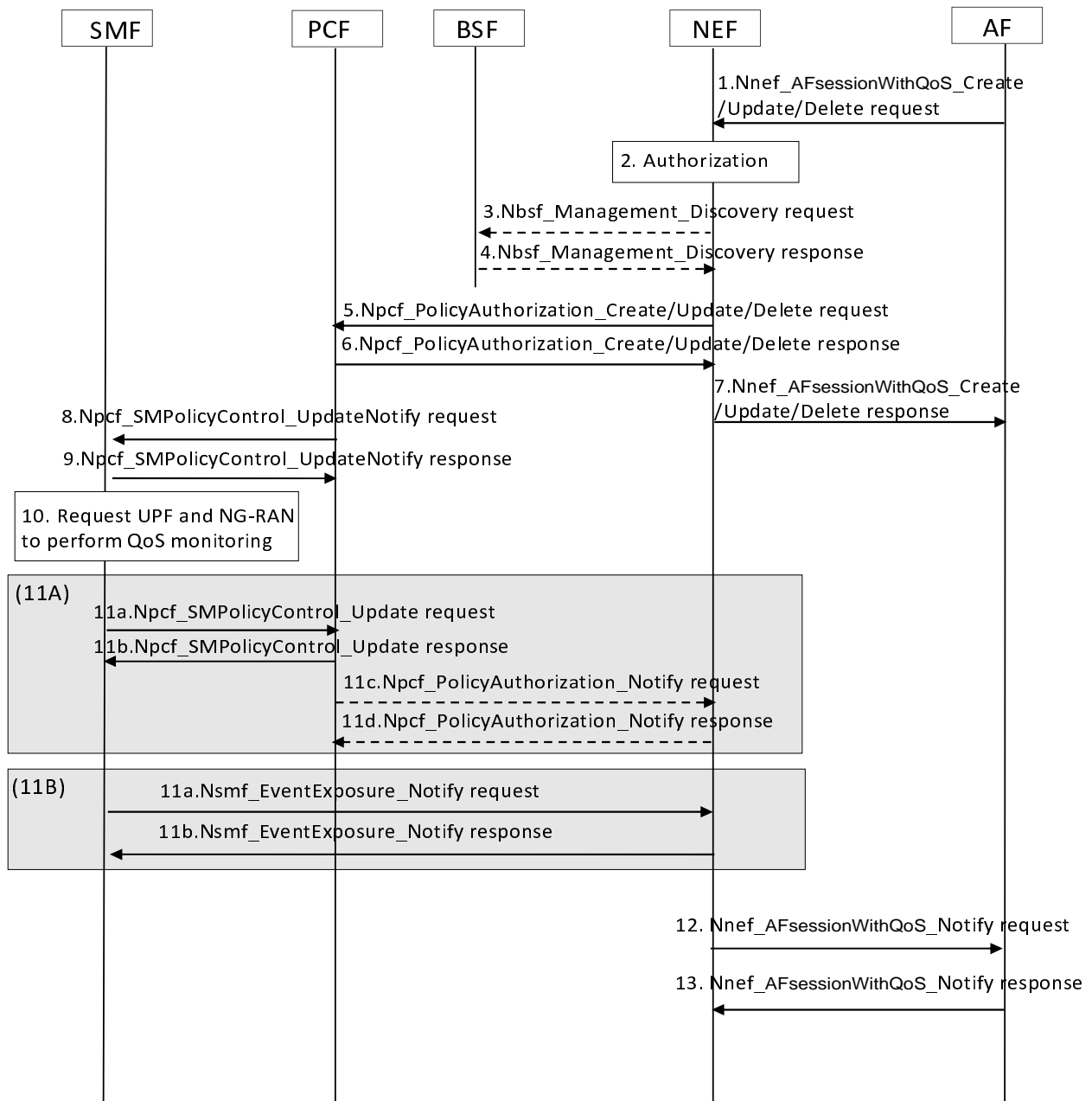
Figure 5.5.9-1: QoS monitoring procedure
