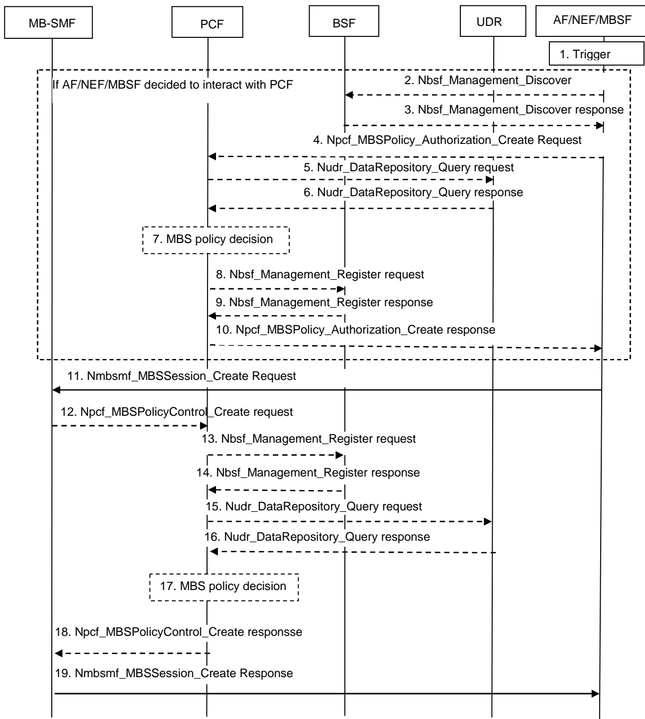
Figure 5.7.2-1: MBS Policy Association Establishment procedure
