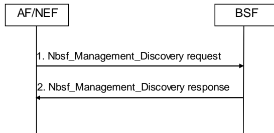
Figure 8.5.4-1 Bind information Retrieval procedure
