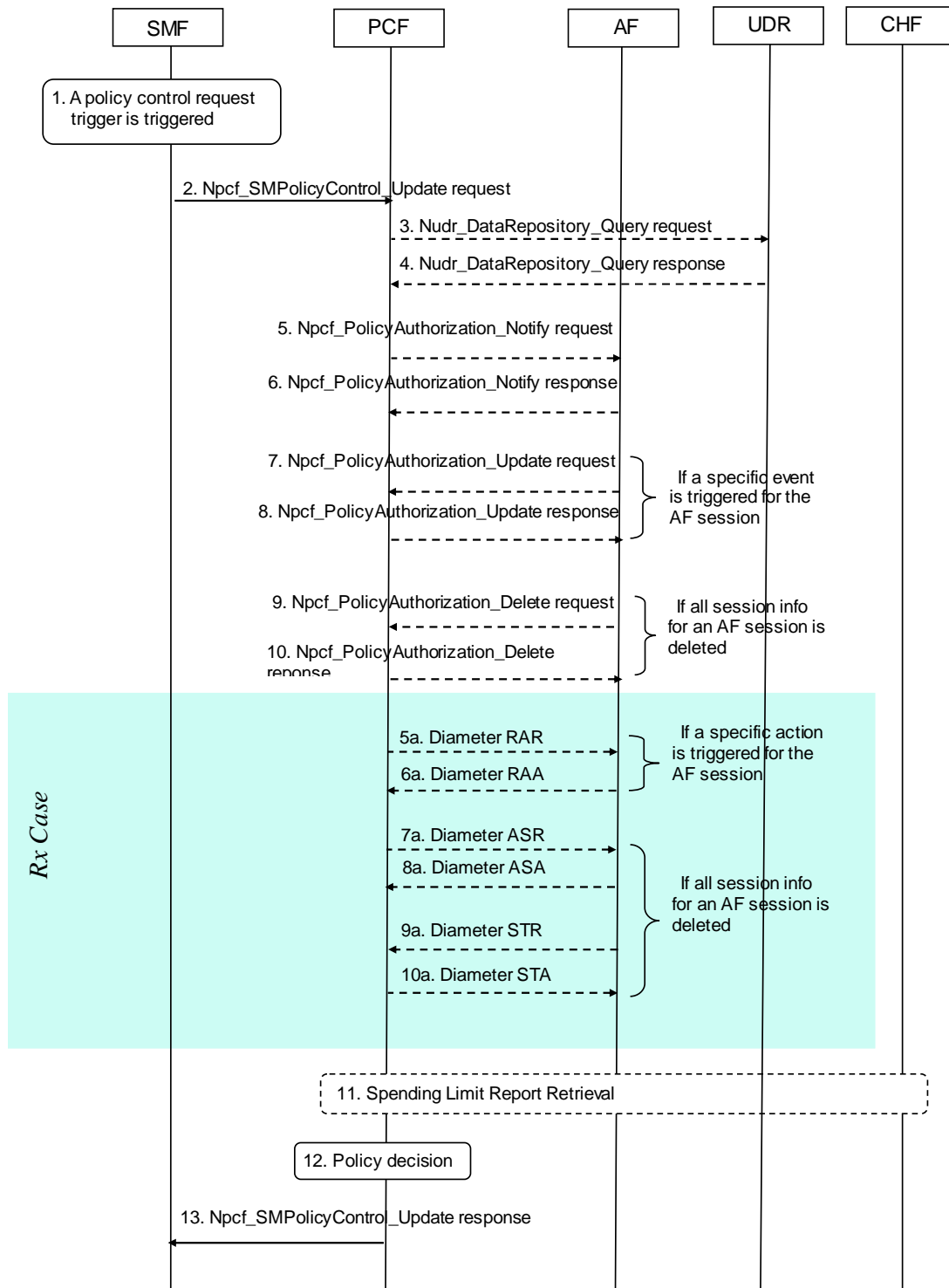
Figure 5.2.2.3-1 SMF-initiated SM Policy Association Modification procedure
