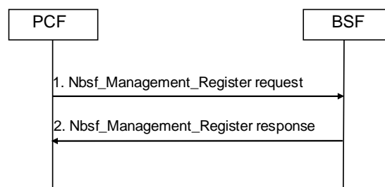
Figure 8.5.2-1 Bind information Creation procedure
