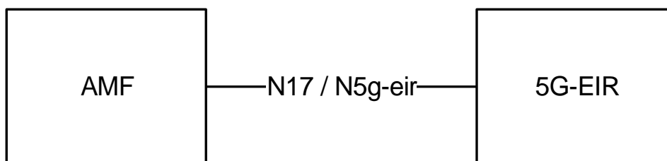
Figure 4-1: Reference Model – N5g-eir
