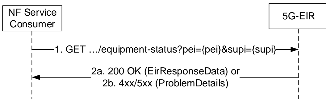
Figure 5.2.2.2-1: PEI status check by the NF Service Consumer
