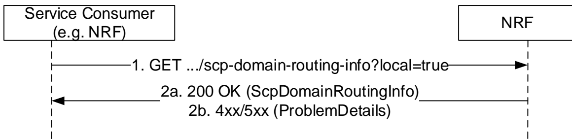
Figure 5.3.2.3-2: Local SCP Domain Routing Information Get
