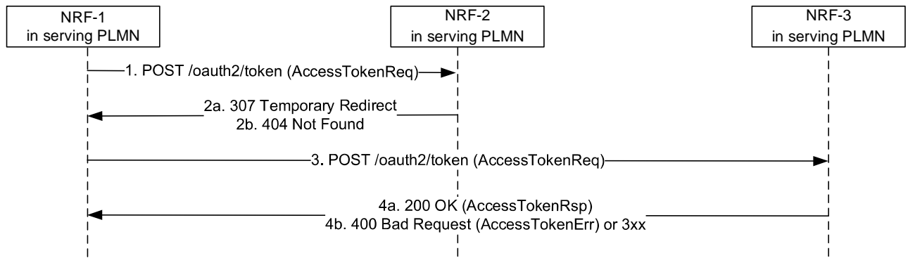
Figure 5.4.2.2.3-1: Access Token Request with intermediate redirecting NRF
