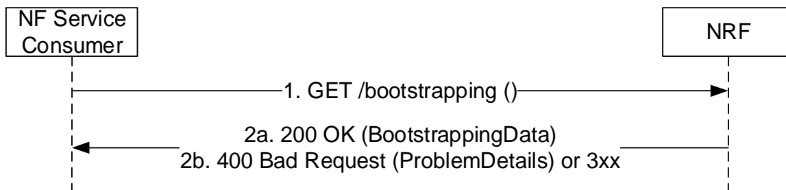
Figure 5.5.2.2.1-1: Bootstrapping Request
