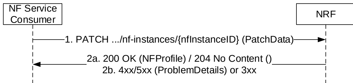
Figure 5.2.2.3.2-1: NF Heart-Beat
