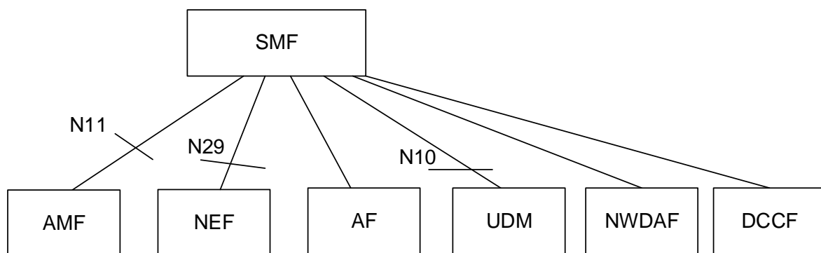
Figure 4.1.2-1: Reference Architecture for the Nsmf_EventExposure Service; SBI representation
