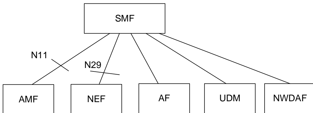
Figure 4.1.2-2: Reference Architecture for the Nsmf_EventExposure Service: reference point representation
