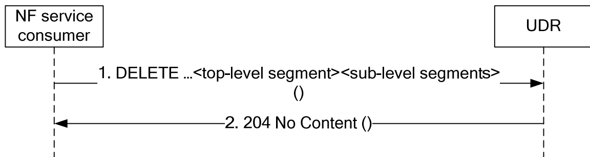
Figure 5.2.2.4.2-1: Deleting Data
