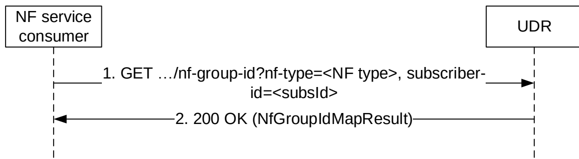
Figure 5.3.2.2.2-1: Retrieving NF-Group Id
