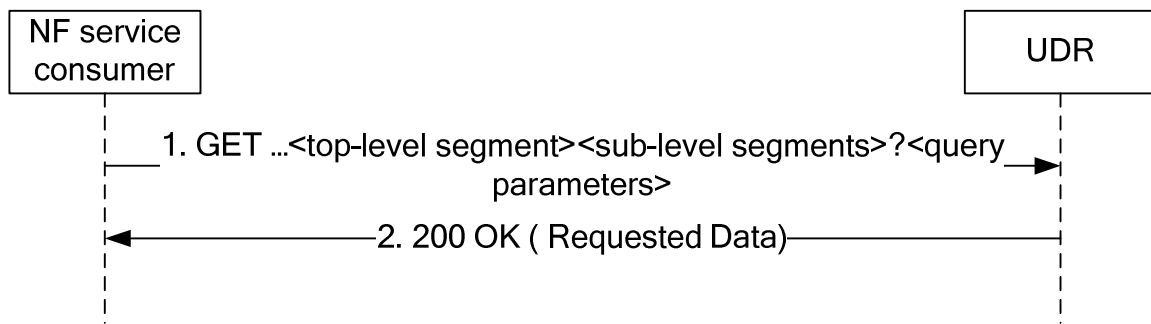
Figure 5.2.2.2-1: Retrieving Data
