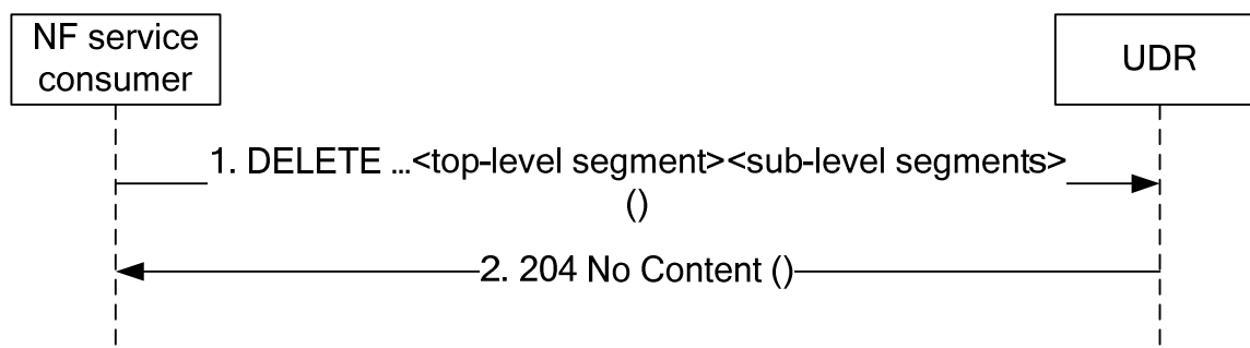
Figure 5.2.2.4.2-1: Deleting Data
