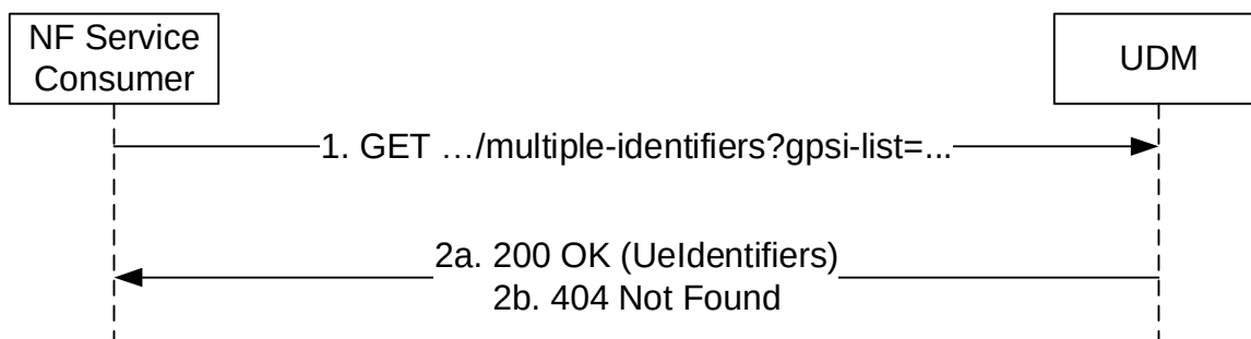
Figure 5.2.2.25: GPSIs Translation
