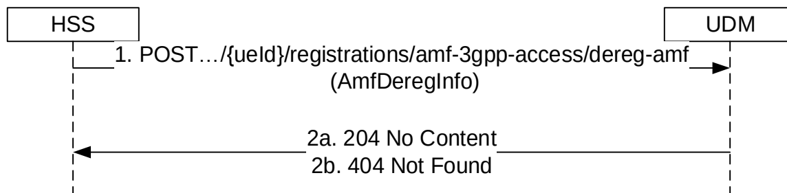
Figure 5.3.2.9.2-1: AMF-Deregistration
