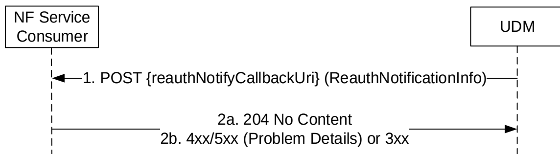
Figure 5.3.2.15.2-1: Reauthentication Notify
