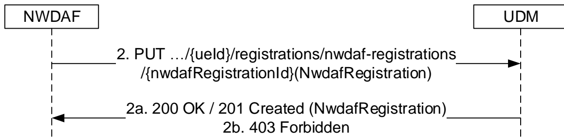
Figure 5.3.2.2.8-1: NWDAF registration
