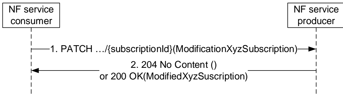
Figure 4.6.2.2.3-1: Modification a subscription using HTTP PATCH
