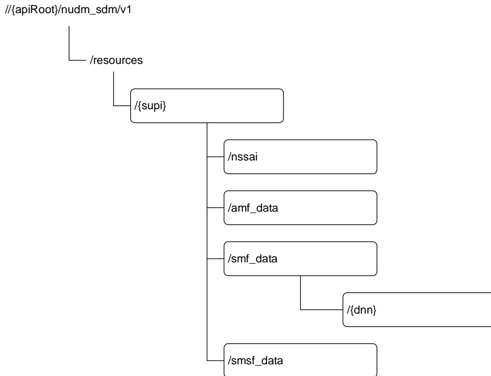
Figure 5.2.1-1: Resource URI structure of the <xyz > API
