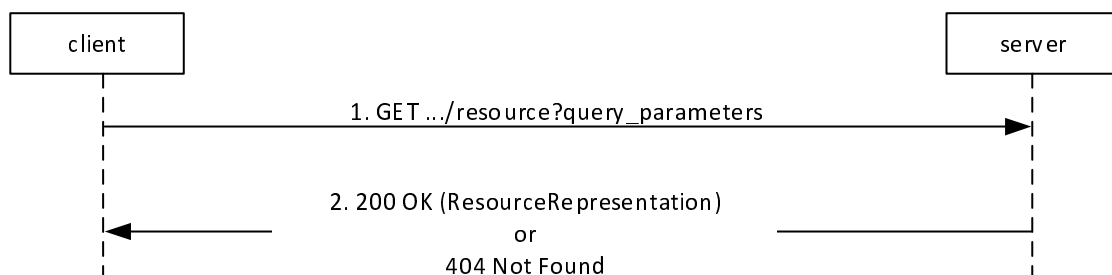
Figure 4.6.1.1.2.2-1 illustrates querying a collection of resources by using query parameters.
