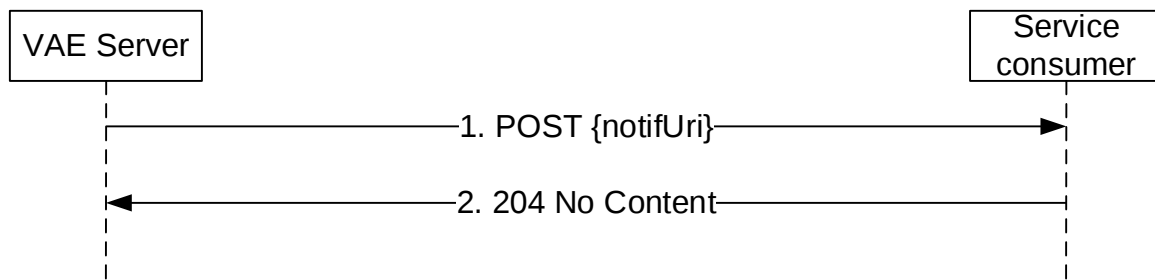
Figure 5.10.2.3.2-1: Notify_PC5ProvisioningRequirement
