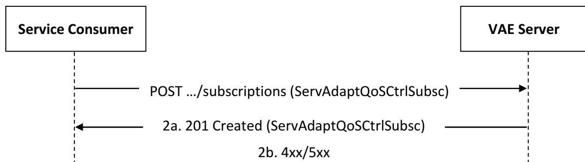
Figure 5.11.2.2.2-1: Procedure for Service Adaptation And QoS Control Subscription Creation
