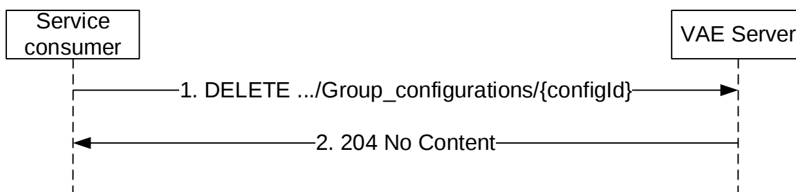
Figure 5.5.2.2.3-1: Termination of Dynamic Group Configuration
