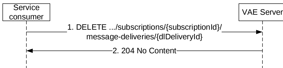
Figure 5.2.2.4.3-1: Termination of Downlink Message Delivery
