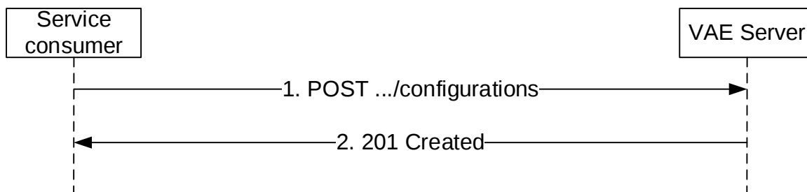
Figure 5.9.2.2.2-1: Request_V2VConfigRequirement
