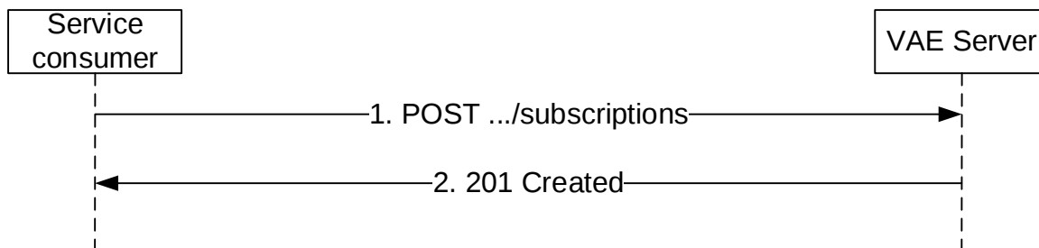
Figure 5.7.2.2.2-1: Subscribe HD Map Dynamic Information
