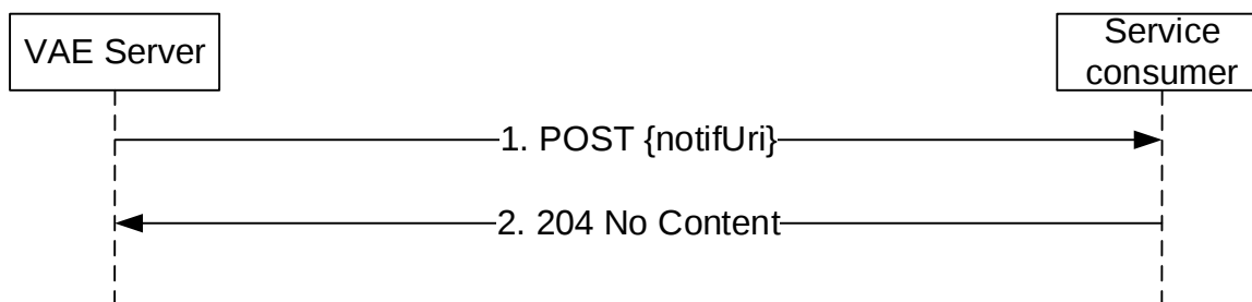
Figure 5.7.2.3.2-1: Notify HD Map Dynamic Information
