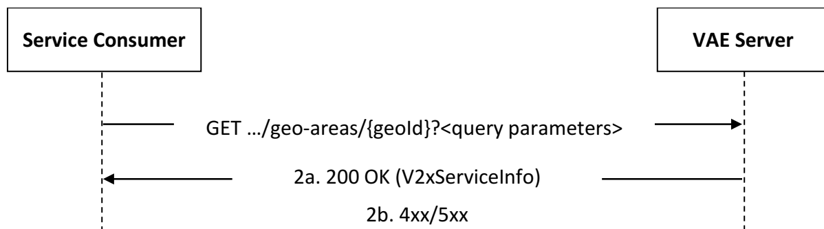
Figure 5.6.2.2.2-1: Query service continuity
