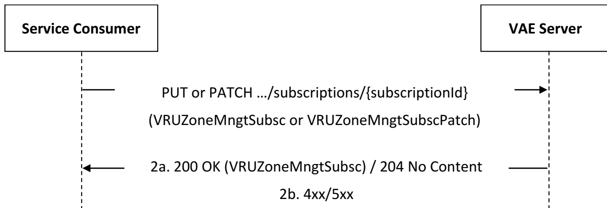
Figure 5.12.2.2.3-1: Procedure for VRU Zone Management Subscription Update
