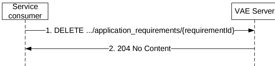
Figure 5.4.2.2.3-1: Termination of Network Resource Reservation
