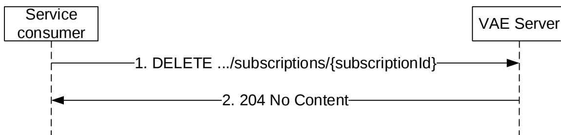
Figure 5.8.2.6.2-1: Terminate Session
