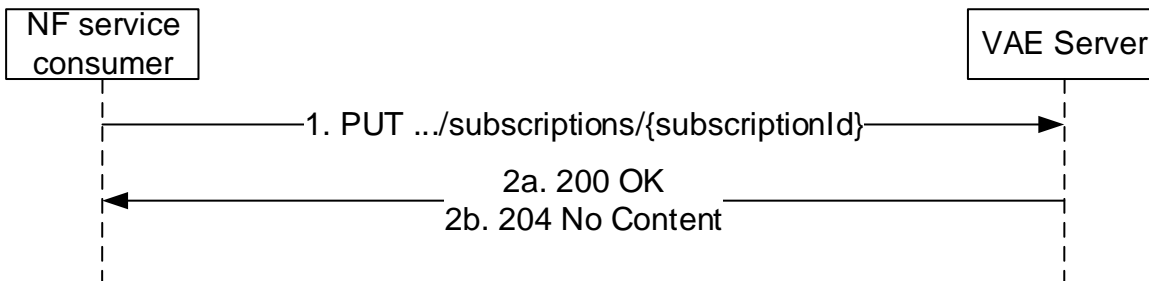
Figure 5.8.2.4.2-1: Update Session
