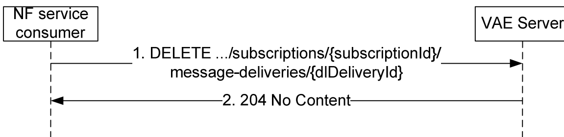
Figure 5.2.2.4.3-1: Termination of Downlink Message Delivery
