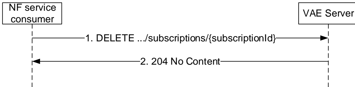
Figure 5.8.2.6.2-1: Terminate Session
