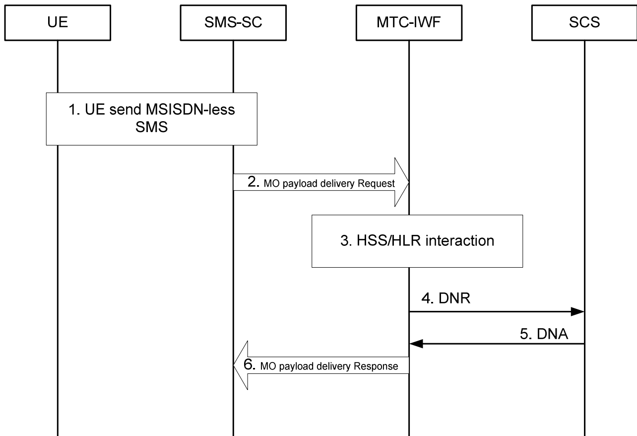
Figure A.9.1: Delivery of a MSISDN-less MO-SMS
