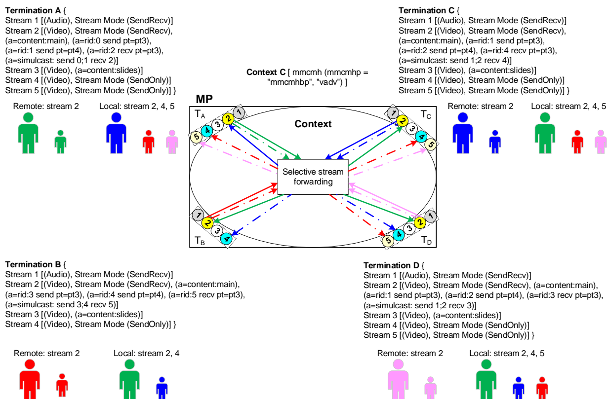
Figure C.2.7.1: Example of MMCMH switching
