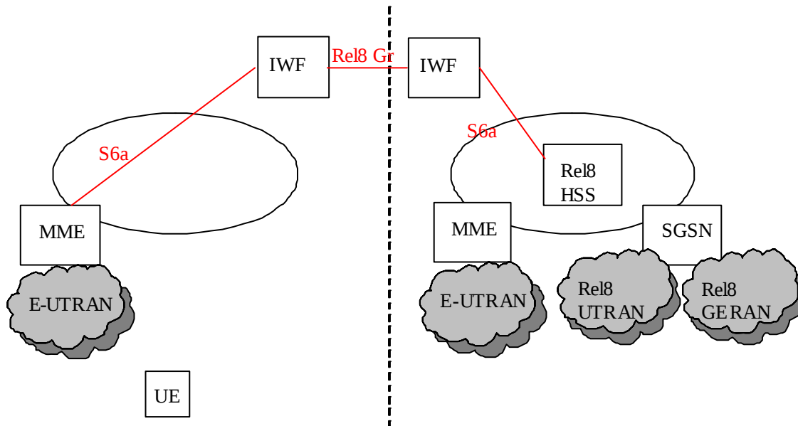
Figure 4.4.2-3 IWF Scenario three network deployment: visited EPS with E-UTRAN only, home EPS with E-UTRAN and UTRAN/GERAN
