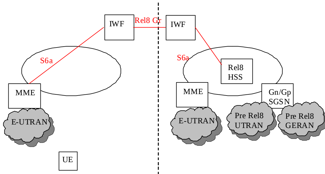
Figure 4.4.2-5 IWF Scenario three network deployment: visited EPS with E-UTRAN only, home ESP with E-UTRAN only and Pre Rel8 UMTS/GPRS
