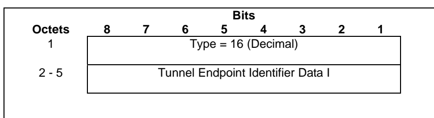
Figure 8.3-1: Tunnel Endpoint Identifier Data I Information Element
