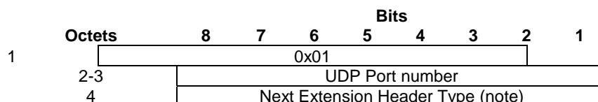
Figure 5.2.2.1-1: UDP Port Extension Header
