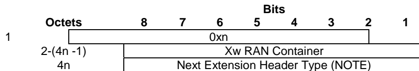
Figure 5.2.2.5-1: Xw RAN Container Extension Header
