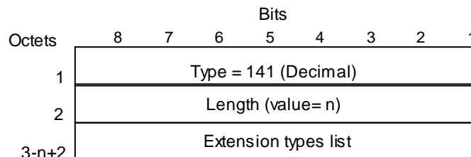
Figure 8.5-1: Extension Header Type List Information Element
