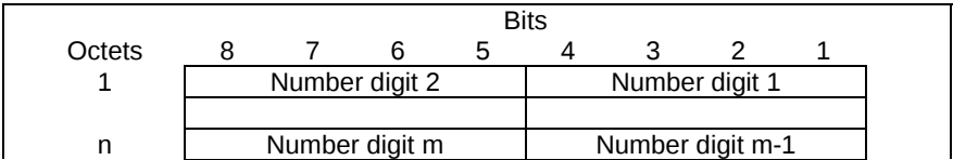
Figure 12.1.1.14-1: Unauthenticated IMSI
