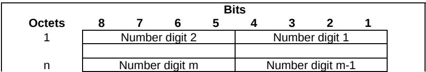
Figure 12.1.1.11-1: MSISDN
