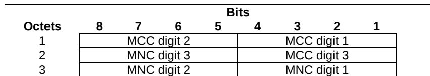
Figure 12.1.1.9-1
