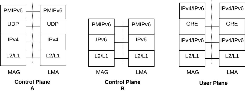
Figure 4.2-1: Protocols stacks for PMIP
