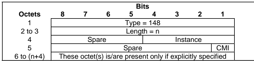
Figure 8.79-1: CSG Membership Indication
