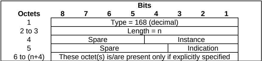
Figure 8.99-1: Action Indication
