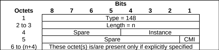
Figure 8.79-1: CSG Membership Indication
