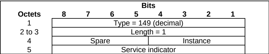
Figure 8.80-1. Service indicator
