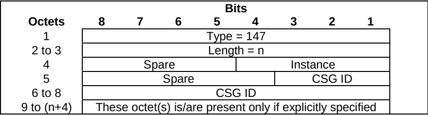
Figure 8.78-1: CSG ID
