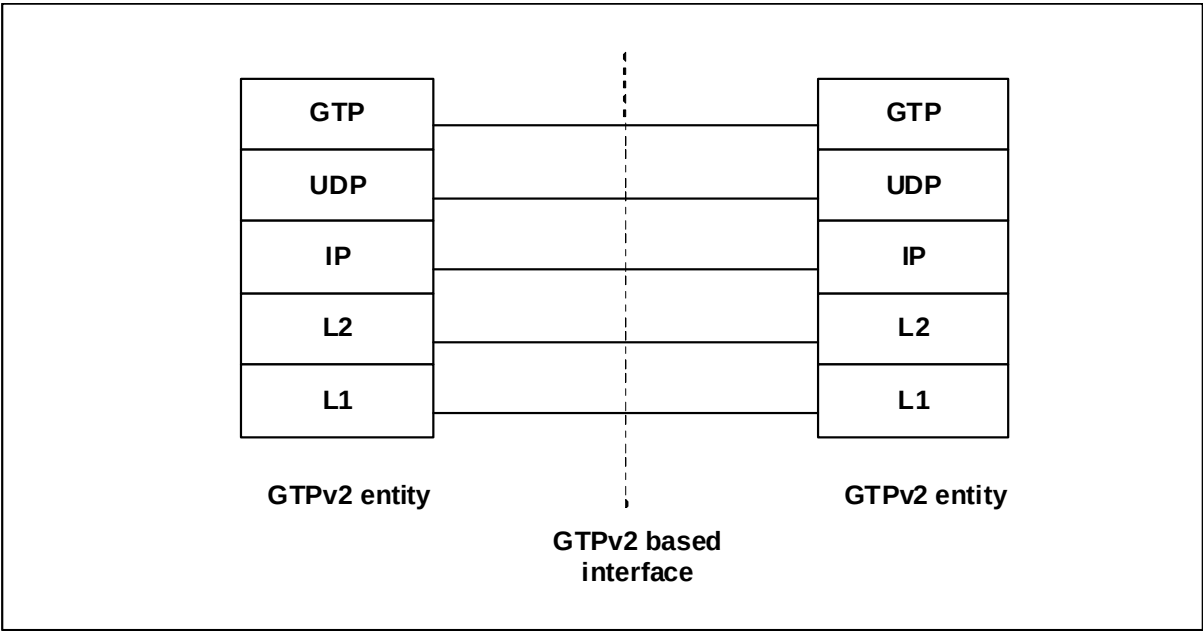
Figure 4.2.0-1: GTPv2 stack
