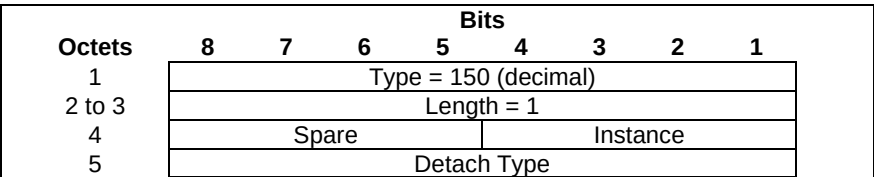
Figure 8.81-1: Detach Type
