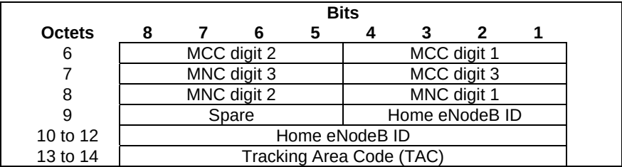
Figure 8.51-3: Target ID for Type Home eNodeB
