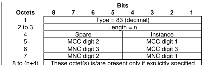
Figure 8.18-1: Serving Network
