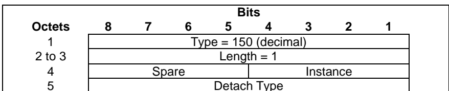
Figure 8.71-1: Detach Type
