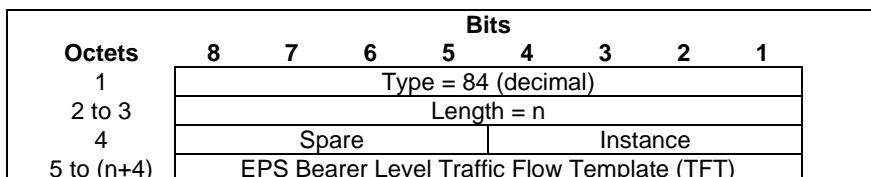
Figure 8.19-1: EPS Bearer Level Traffic Flow Template (Bearer TFT)
