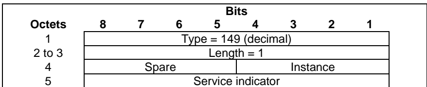
Figure 8.70-1. Service indicator
