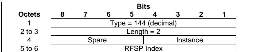
Figure 8.69-1. RFSP Index
