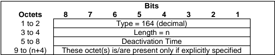
Figure 8.2.122-1: Deactivation Time
