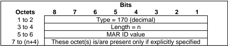
Figure 8.2.123-1: MAR ID
