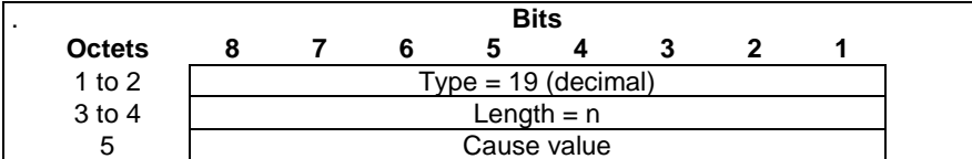
Figure 8.2.1-1: Cause
