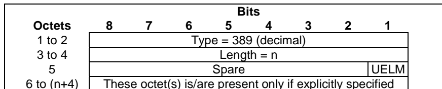
Figure 8.2.272-1: Reporting Control Information
