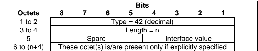
Figure 8.2.24-1: Destination Interface
