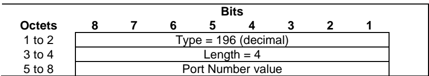
Figure 8.2.141-1: Port Number
