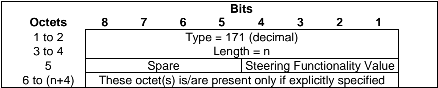
Figure 8.2.124-1: Steering Functionality
