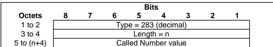
Figure 8.2.191-1: Called Number
