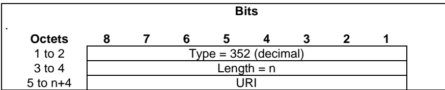
Figure 8.2.244 -1: URI
