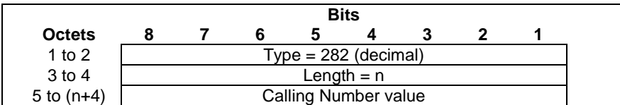
Figure 8.2.190-1: Calling Number
