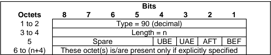
Figure 8.2.59-1: Usage Information
