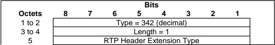
Figure 8.2.234-1: RTP Header Extension Type
