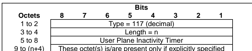
Figure 8.2.83-1: User Plane Inactivity Timer
