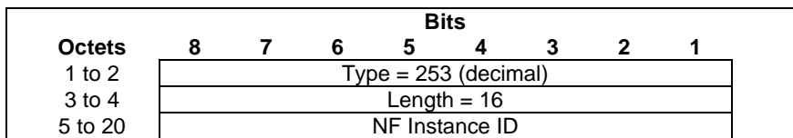
Figure 8.2.175-1: NF Instance ID
