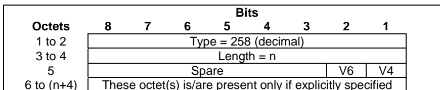
Figure 8.2.177-1: IP version
