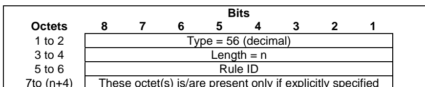
Figure 8.2.36-1: PDR ID
