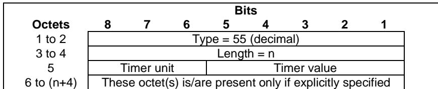
Figure 8.2.35-1: Timer
