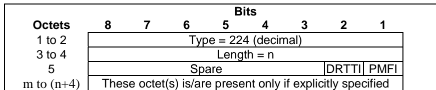
Figure 8.2.156-1: PMF Control Information
