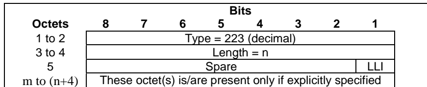
Figure 8.2.155-1: ATSSS-LL Control Information
