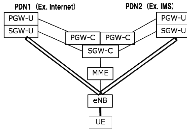
Figure B.2.4 -1: SGW-U/PGW-U colocation with Control and User Plane Separation
