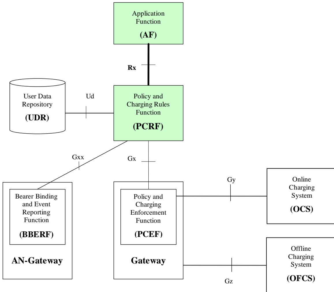
Figure 4.2: Rx reference point at the Policy and Charging Control (PCC) architecture with UDR
