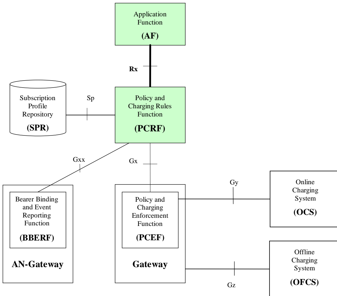
Figure 4.1: Rx reference point at the Policy and Charging Control (PCC) architecture with SPR
