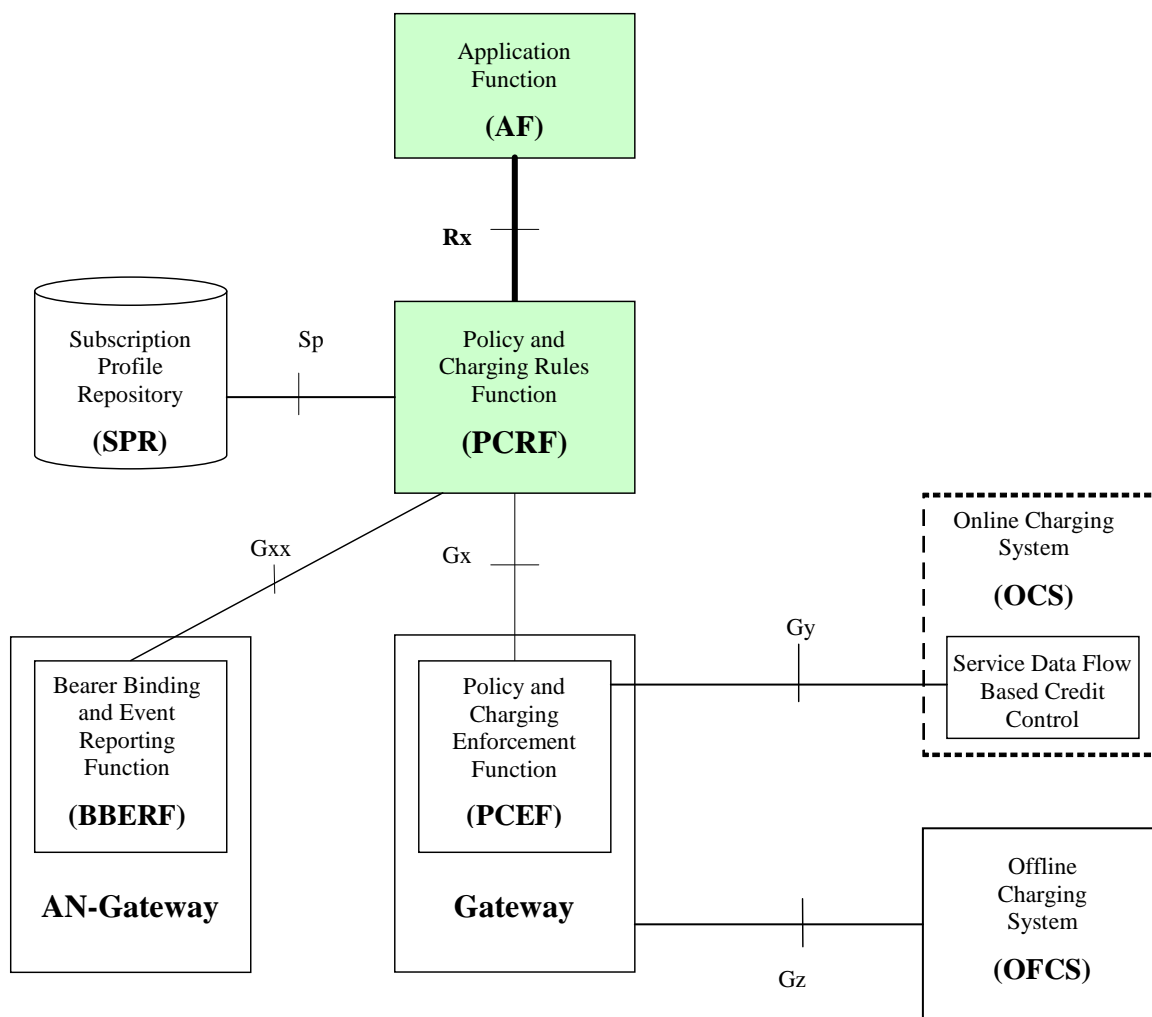
Figure 4.1: Rx reference point at the Policy and Charging Control (PCC) architecture
