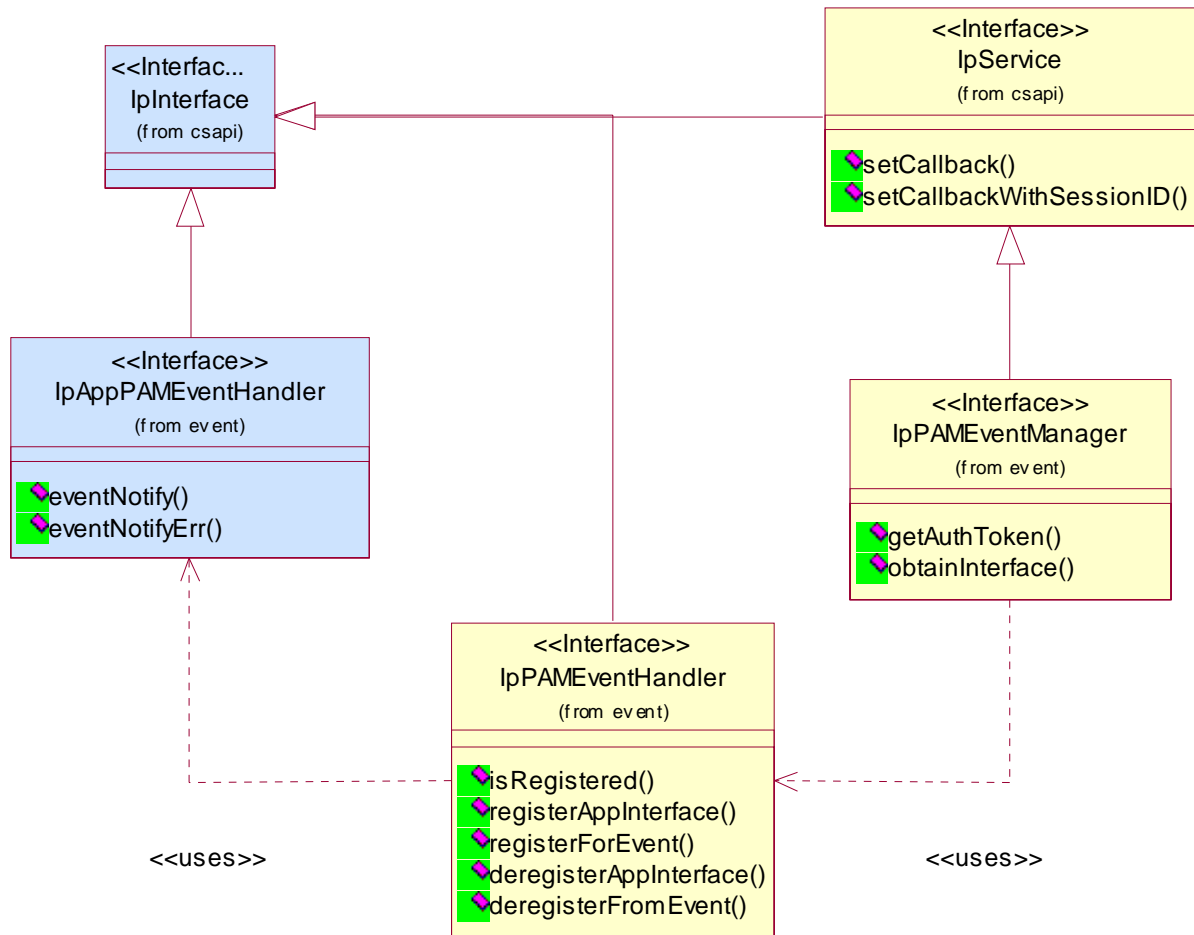
Figure: PAM Event Management Service
